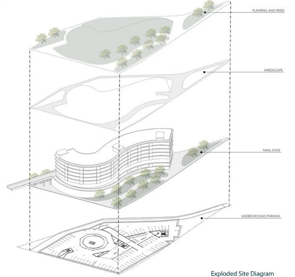
Exploded Site Diagram
