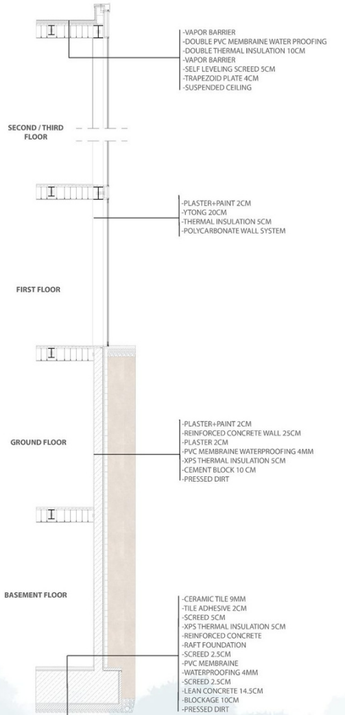
01 / Construction section
