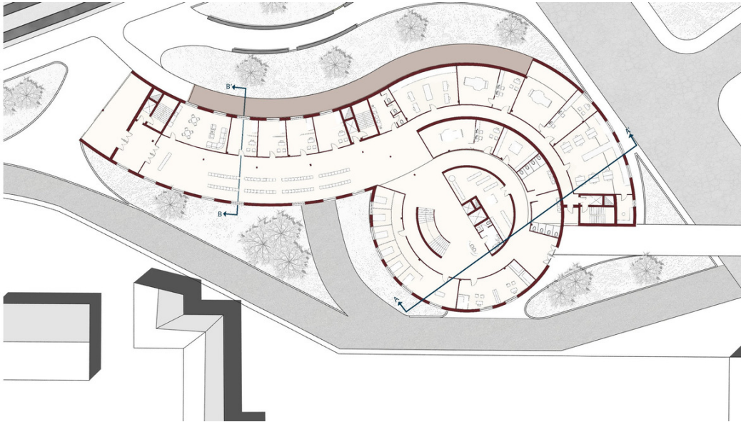
01 / Ground-floor plan
